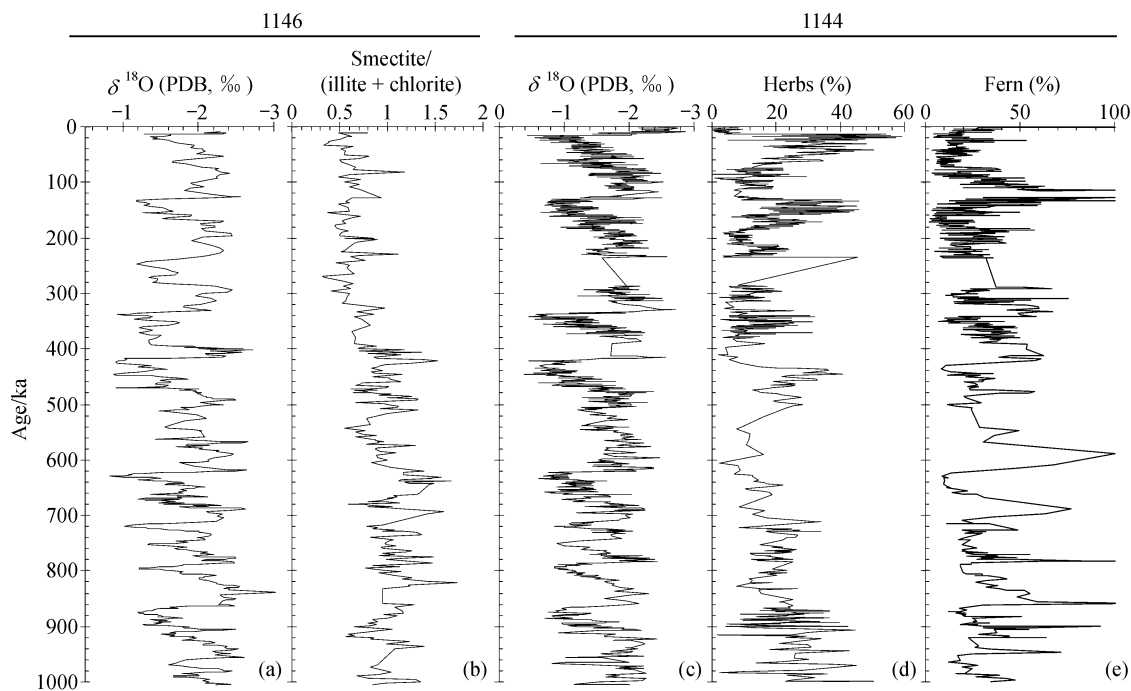
Fig. 3. Variations of monsoon proxies in the northern SCS in the last one million years. Site 1146: (a) planktonic \delta^{18}\text{O} ; (b) ratio of smectite/(illite+chlorite); Site 1144: (c) planktonic \delta^{18}\text{O} ; (d) herbs%; (e) ferns% (percentages in the total pollen sum).
