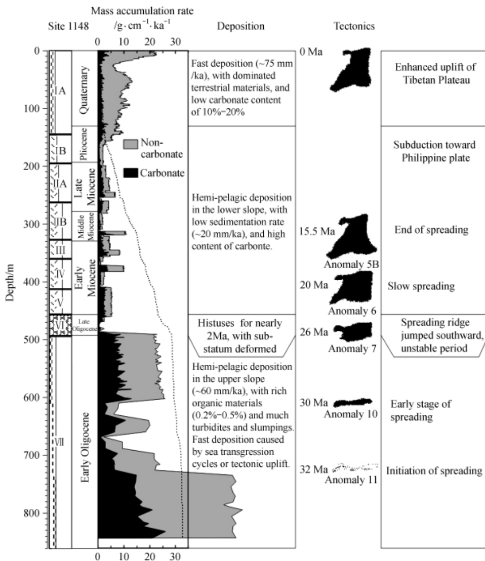
Fig. 7. Seafloor spreading and depositional evolution of the SCS. The accumulation rates modified from [4], the age model for sea floor spreading adjusted according to [43, 44].
