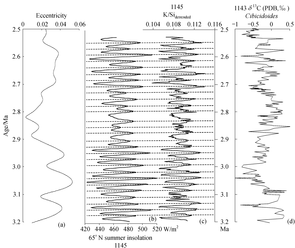
Fig. 2. Orbital forcing of the summer monsoon variations in the SCS in the late Pliocene (3.2–2.5 Ma). (a) Eccentricity [29] ; (b) summer insolation at 65°N; (c) K/Si ratios at Site 1145 [27] ; (d) benthic \delta^{13}\text{C} at Site 1143.
