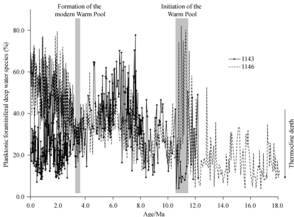
Fig. 9. Downcore variations in percentage of deep dwelling planktonic foraminifers since the Miocene at Sites 1146 and 1143, showing N-S contrasts in the history of thermocline changes in the SCS [50] .
