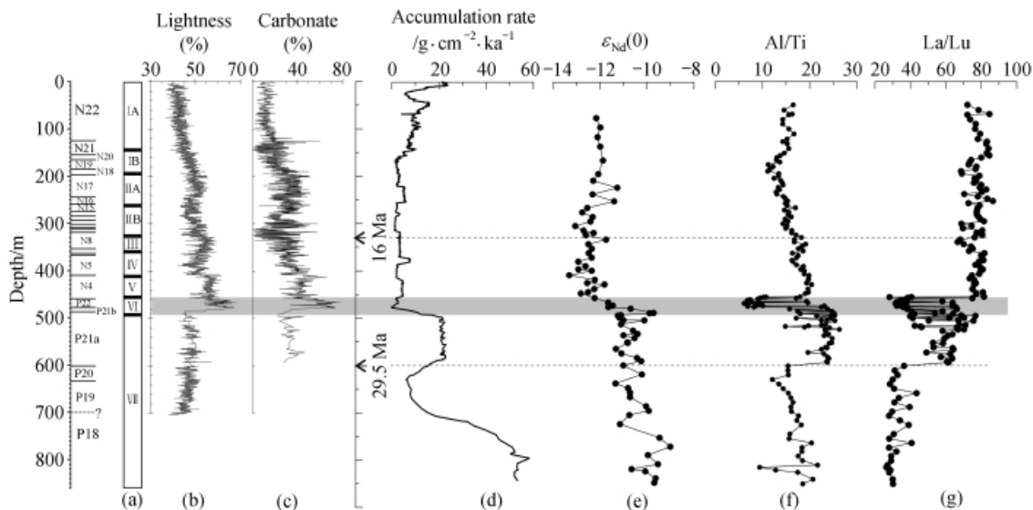
Fig. 6. Stratigraphy, lithology and geochemistry at ODP Site 1148. (a) Lithological units, the Roman denotes unit number, and unit VI is slumping deposits; (b) color reflectance, L^* % [51] ; (c) \text{CaCO}_3 % [42] ; (d) accumulation rate; (e) \epsilon_{\text{Nd}}(0) ; (f) Al/Ti ratio; (g) La/Lu ratio.
