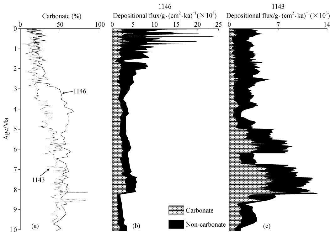
Fig. 8. Comparison of the accumulation rate and sediment composition since 10 Ma between the southern (Site 1143) and northern SCS (Site 1146). (a) \text{CaCO}_3\% , modified from [4]; (b) accumulation rate at Site 1146; (c) accumulation rate at Site 1143, modified from [4].
