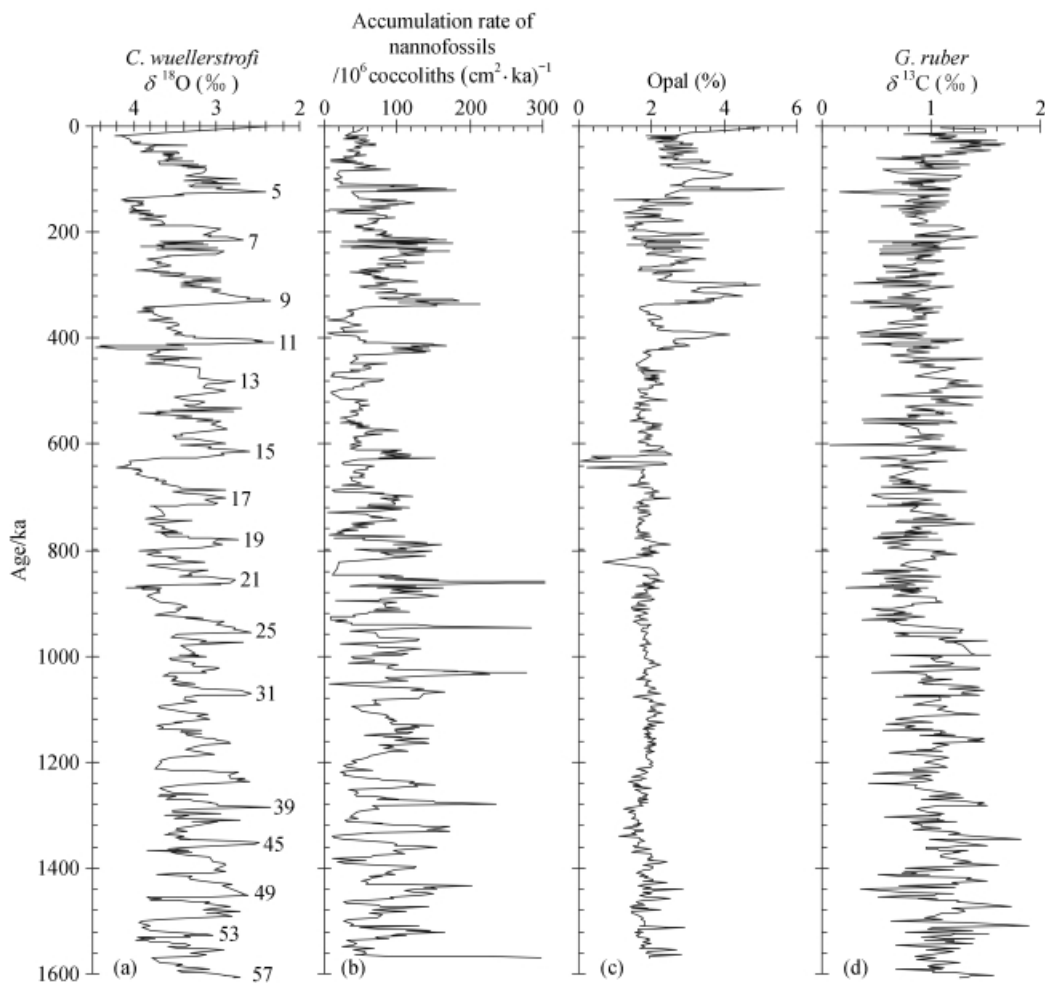
Fig. 4. Variations of monsoon proxies at Site 1143 in the southern SCS since 1.6 Ma. (a) Benthic \delta^{18}\text{O} ; (b) accumulation rate of nannofossils [34] ; (c) opal% [35] ; (d) planktonic Globigerinoides ruber \delta^{13}\text{C} [28] .
