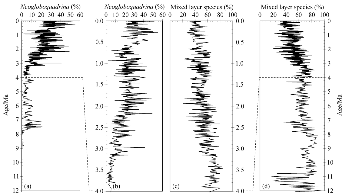
Fig. 1. Downcore variations of planktonic foraminifers% at Site 1146 since 12 Ma. (a) and (b) Neogloboquadrina dutertrei %; (c) and (d) percentage of the mixed layer shallow water species.
